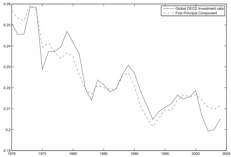
Figure 3: First Principal Component
