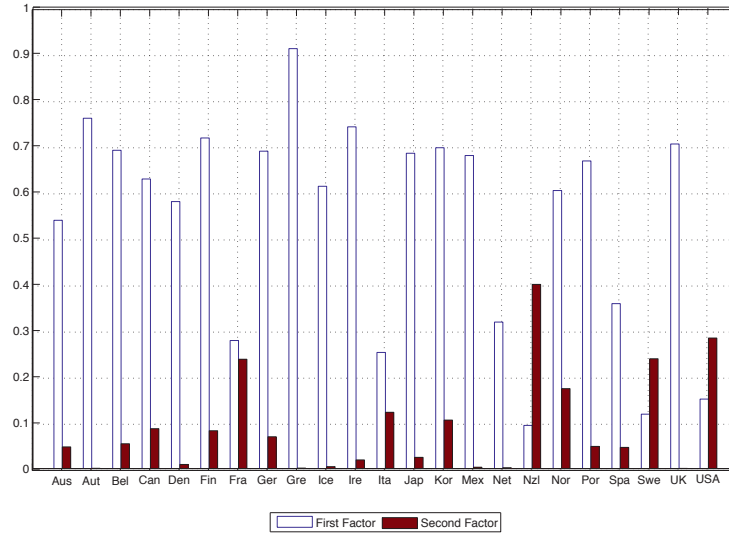
Figure 1: Domestic Saving. Percentage of variance explained by the first two factors.
