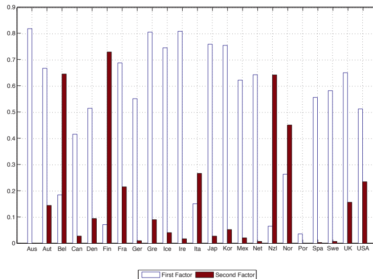
Figure 2: Domestic Investment. Percentage of variance explained by the first two factors.
