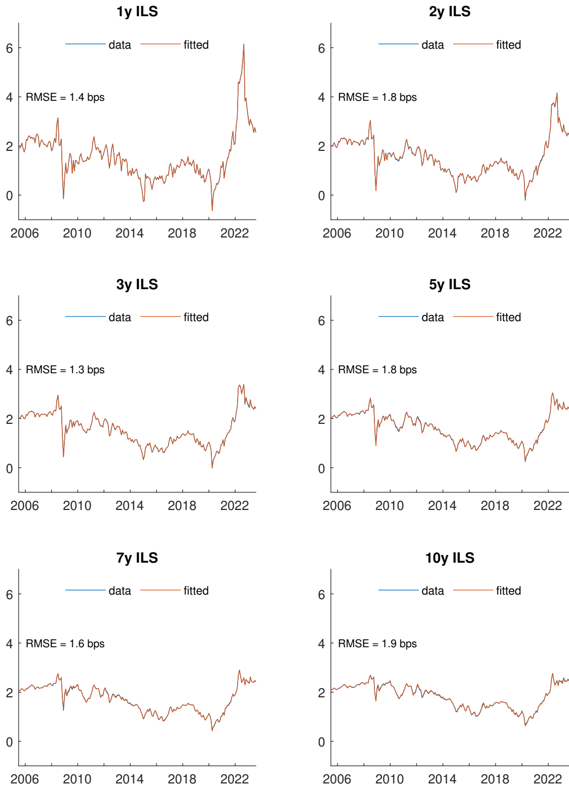
Figure 3: Model fit to ILS rates
