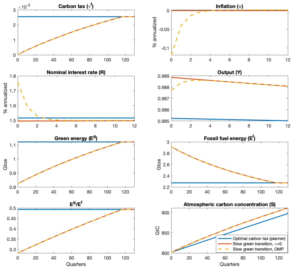
Figure 3: Transitions in baseline model
