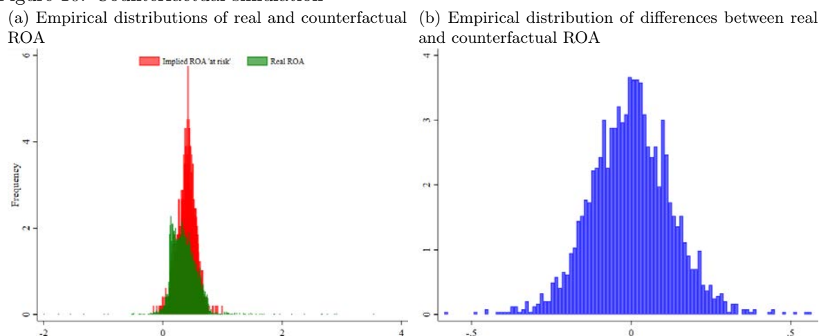
Figure 10: Counterfactual simulation
