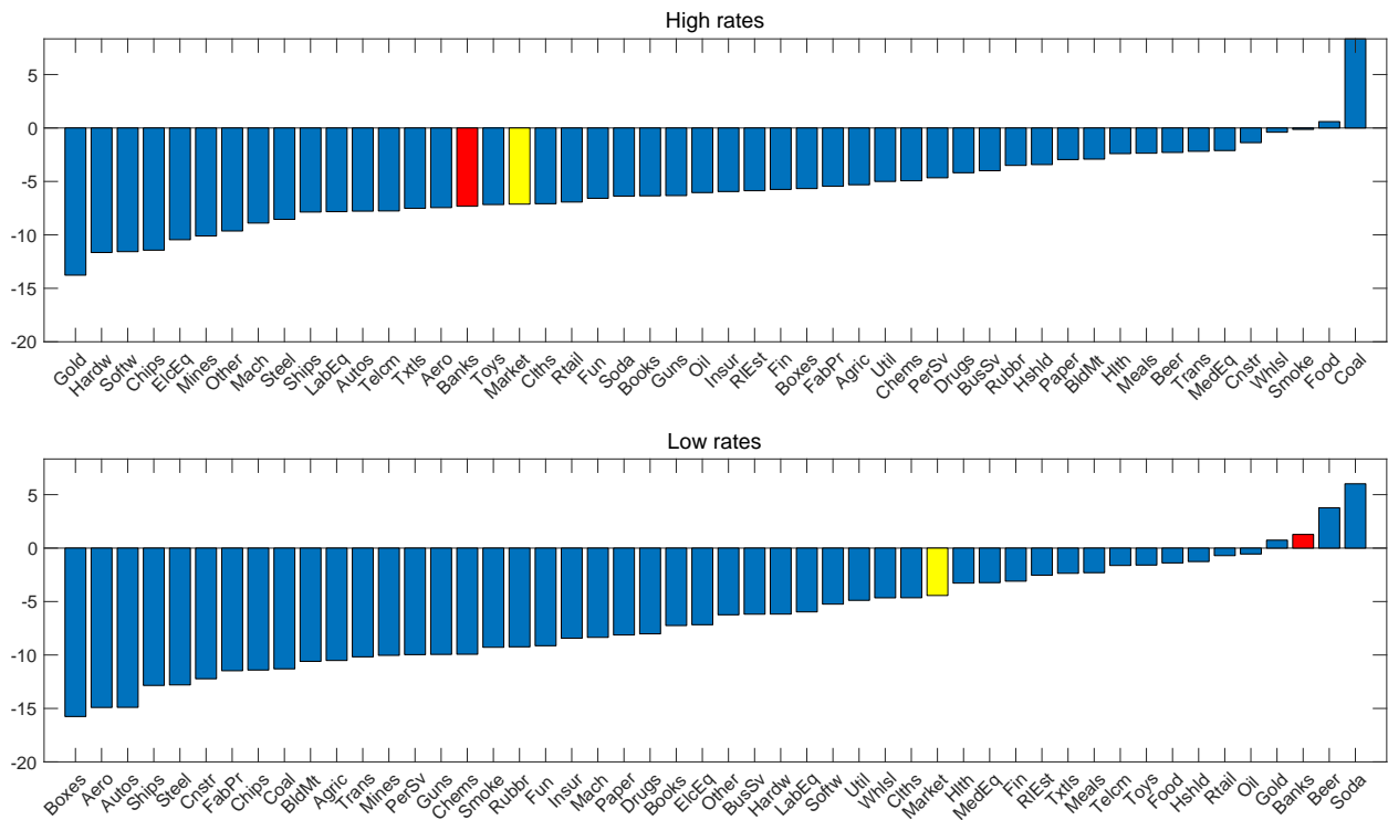
Figure 21: Response of Fama-French's 49 industry portfolios and market portfolio to a 100 bps shock to the Fed funds rate.
