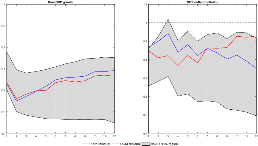
(b) Conditional Forecast
