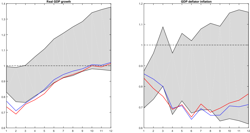
(a) Unconditional Forecast
