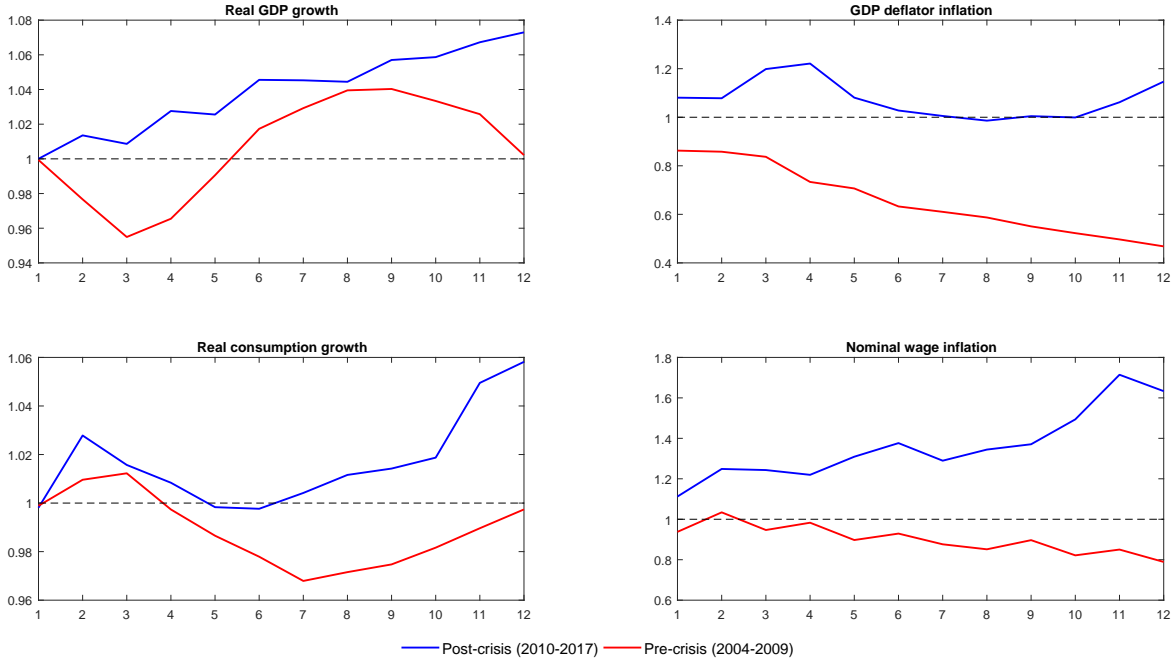
Figure D.15: Comparing the forecast performance over time and across different degrees of anchoring
