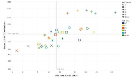
a) Comparison of emissions (GHGs) and MSA loss caused by climate change, both normalised by sectoral revenues
