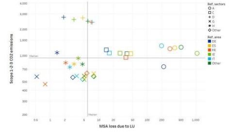
b) Comparison of emissions (GHG) and MSA loss caused by LU, both normalised by sectoral revenues
