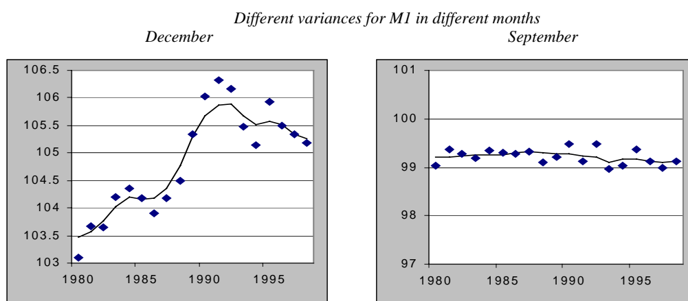
Chart 2.2.2: Seasonal factors (straight line) and seasonal times (irregular) for M1 (December to September)
