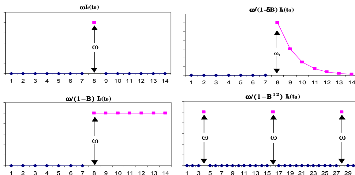
Chart 2.4.1: Polynomials for additive outlier, transient change, level shift and seasonal outlier.
