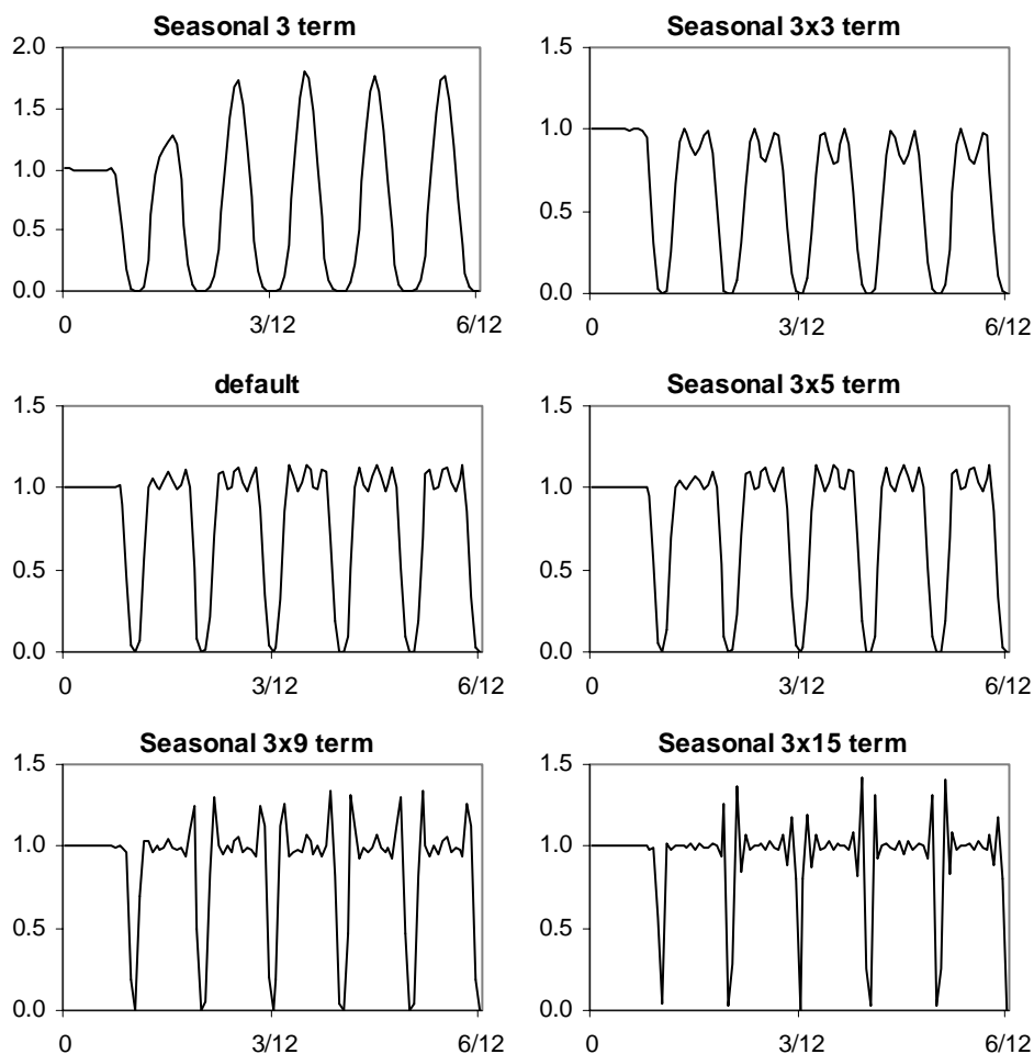
Chart 4.2.2: Squared gain of different seasonal adjustment filters of X-11 using the 13-term Henderson trend
