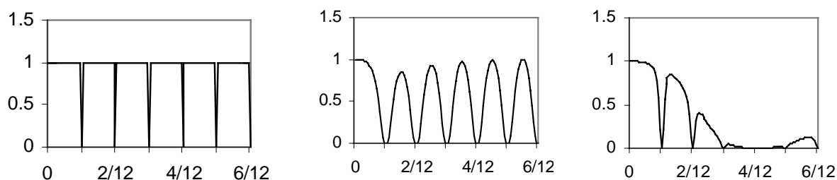
Chart 4.2.3: Different seasonal adjustment filters in SEATS
