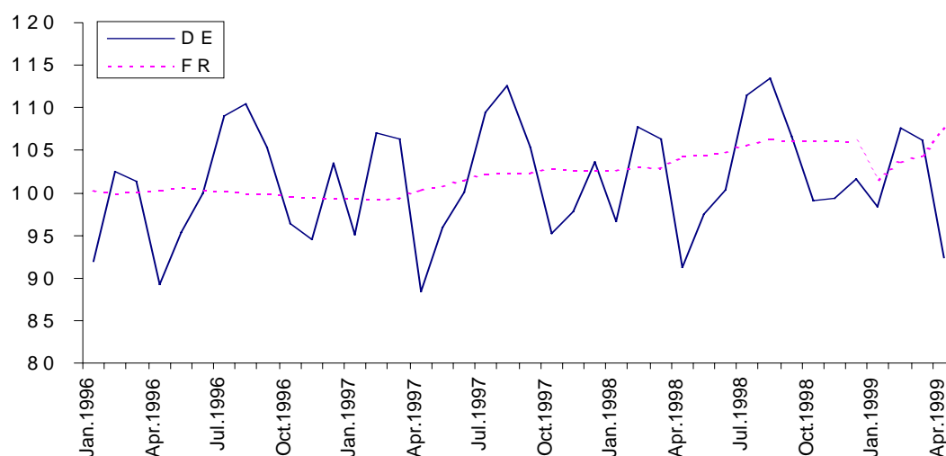
Chart 3.2.1: Price index for package holidays (France and Germany)
