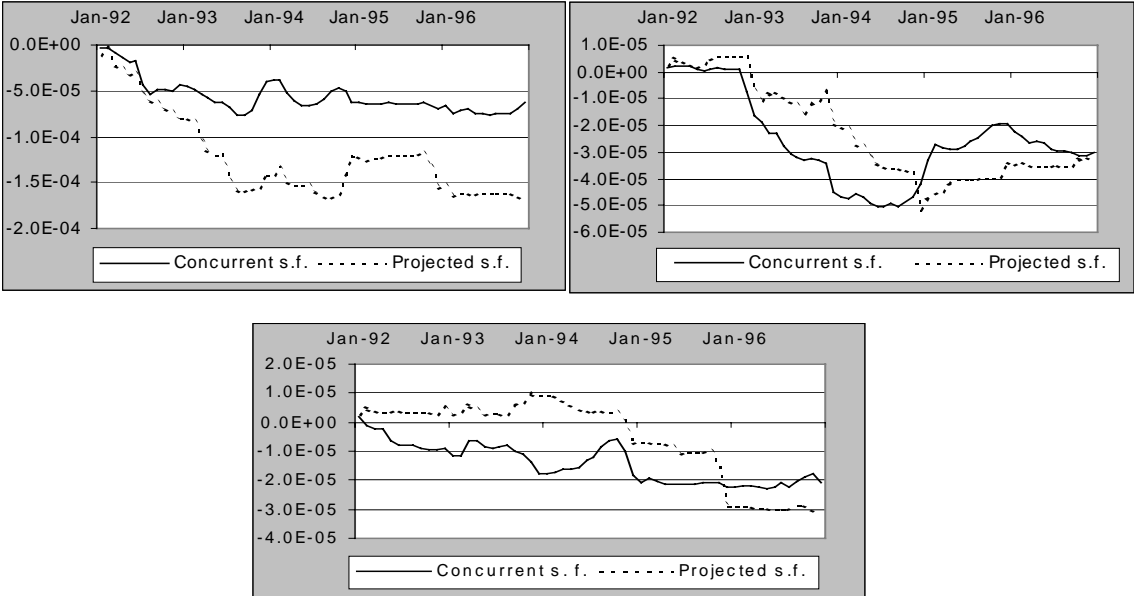
Chart 2.2.1: Difference of the summed squared revisions between X-12-ARIMA and X-11 (M1, M2-M1, M3)
