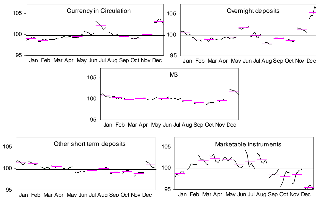
Chart 3.1.1: Seasonal factors (multiplied by 100) for the components of euro area M3
