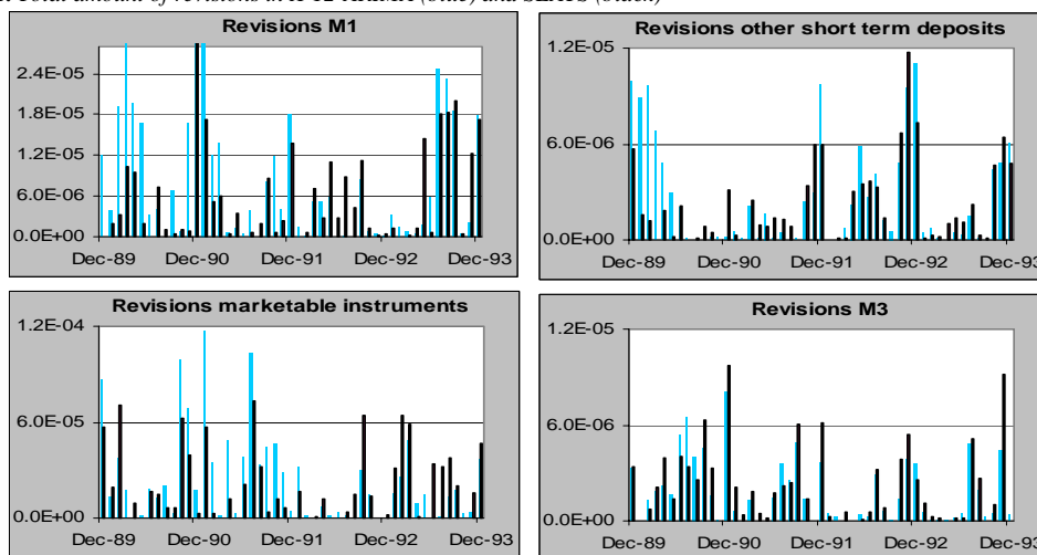
Chart 4.3.1: Total amount of revisions in X-12-ARIMA (blue) and SEATS (black)
