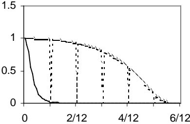
Chart 4.2.4: Squared gains of different trend filters of the AIRLINE model
