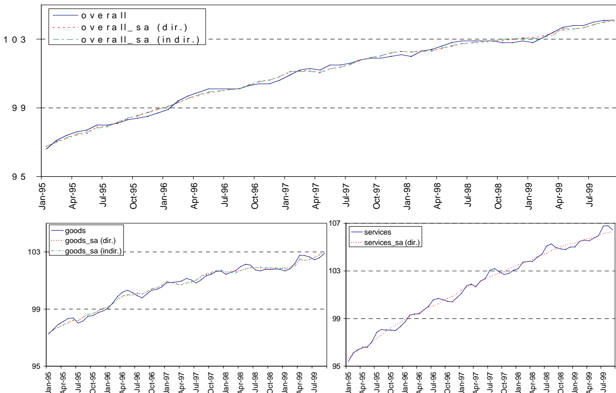
Chart 3.2.3: Raw and seasonally adjusted series for the euro area overall index, goods and services.
