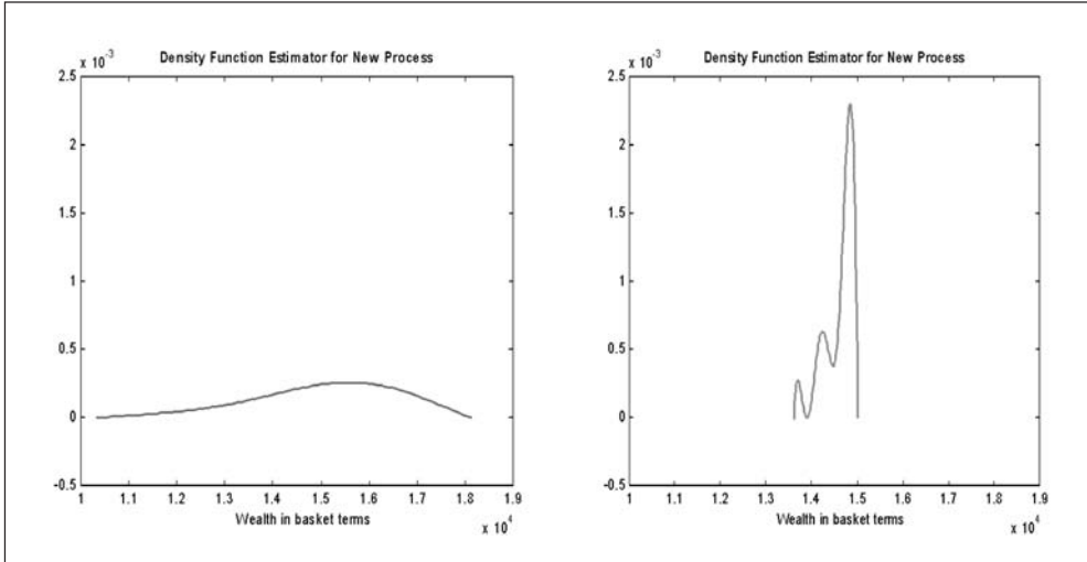
Figure 3: Density functions before and after shaping
