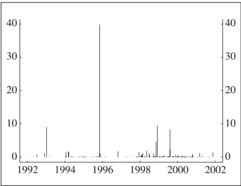
Figure 1: Operational risk losses, Type 1, n = 162
