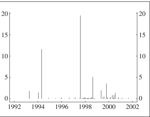
Figure 2: Operational risk losses, Type 2, n = 80
