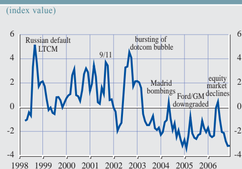
Chart D.1 Composite risk appetite indicator
