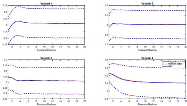
Figure 3: Conditional forecast from a medium VAR with one soft constraint. The thick black line is the posterior median estimate of the conditional forecast using the proposed precision-based method. The thick red line is the posterior median estimates of the conditional forecast using the Waggoner and Zha (1999) method. The thick blue line is the posterior median estimates of the conditional forecasting using the Andersson, Palmqvist, and Waggoner (2010) (APW) method. The dash lines are the corresponding 68 per cent credible intervals for all three methods.
