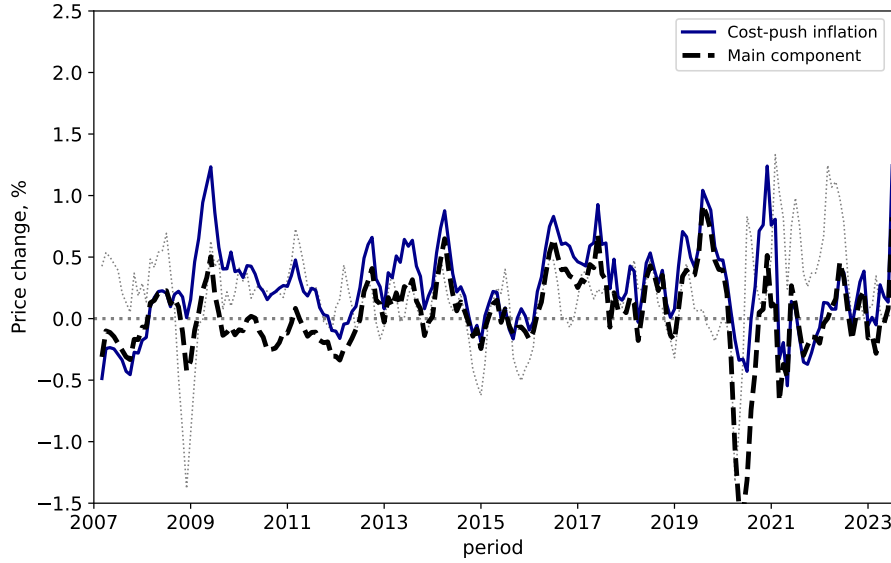
Figure 7: Cost-push inflation and main component
