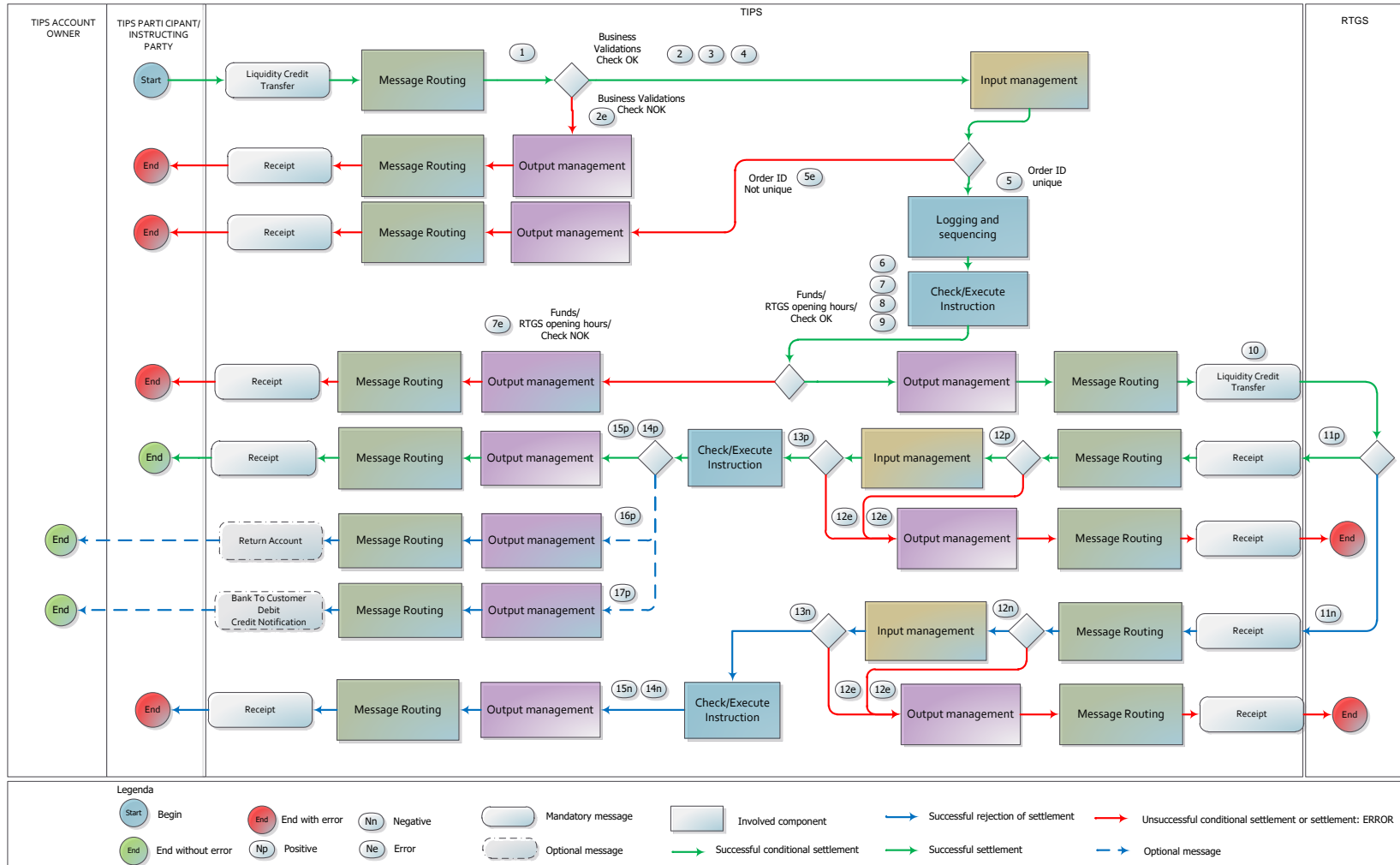
Figure 153 – Outbound Liquidity Transfer Order flow
