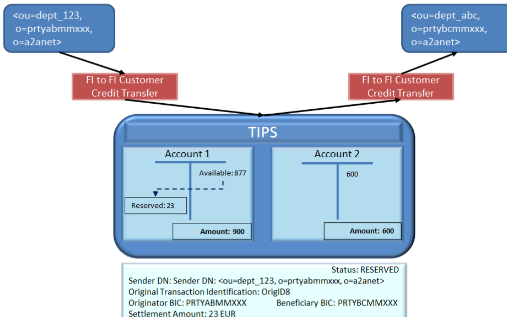
Figure 55 – Delayed Beneficiary-side answer: reservation of funds
