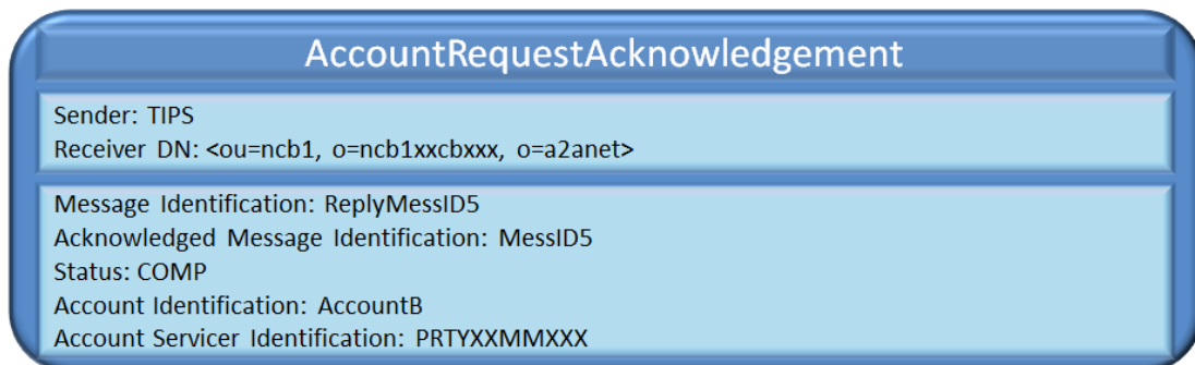
Figure 235 – Successful unblock of an Account: AccountRequestAcknowledgement
