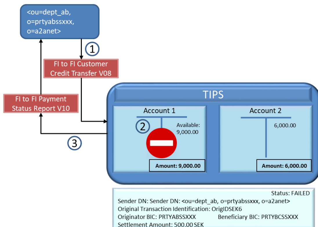
Figure 84 – Blocked account error: transaction failed
