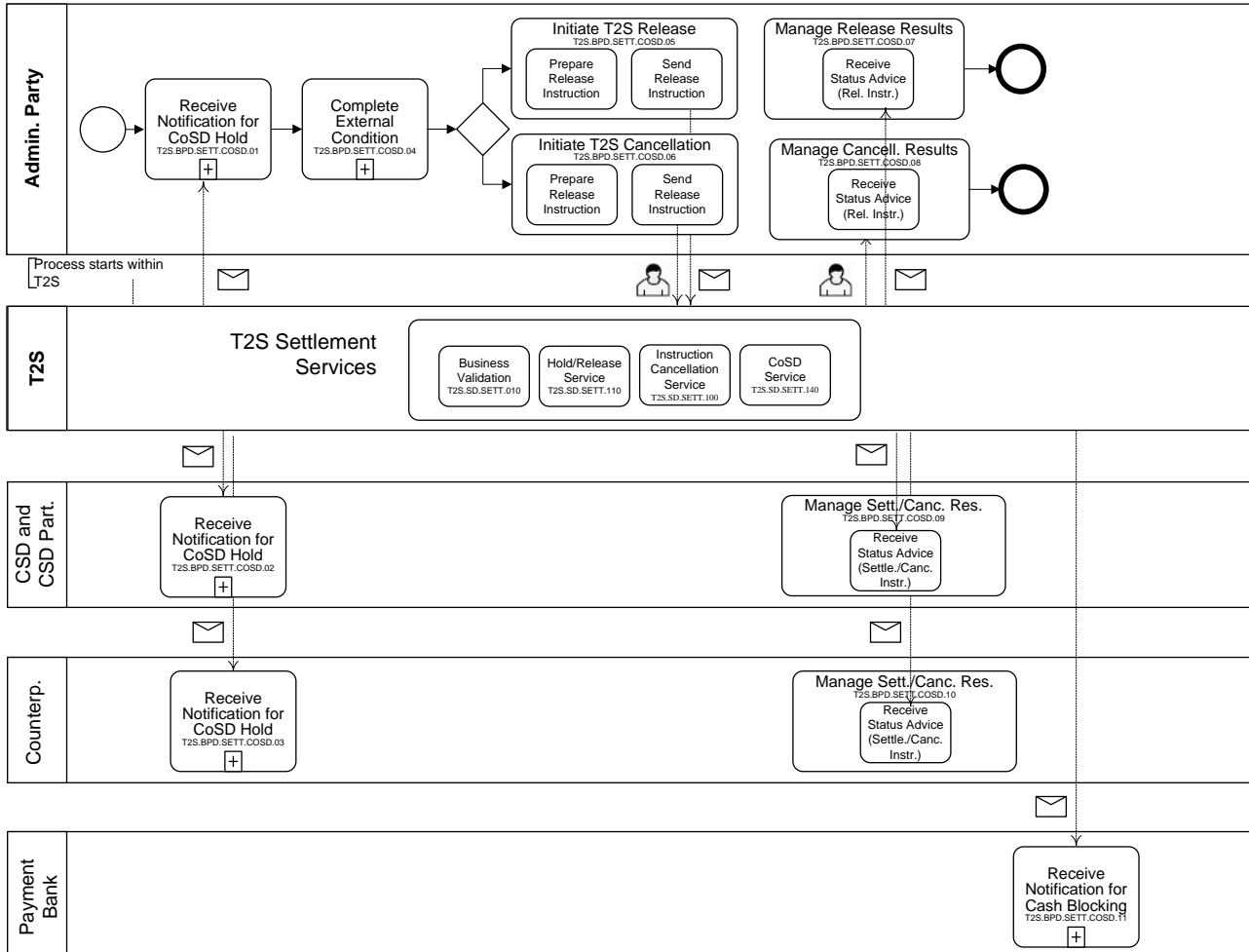
2 Figure 3-3: Business Process Diagram [T2S.BPD.SETT.COSD]
