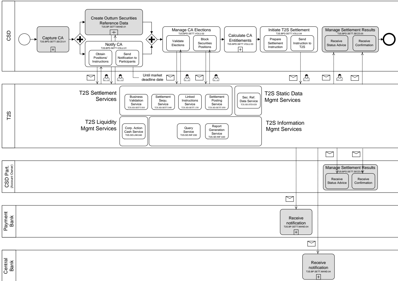
2 Figure 5-9: Business Process Diagram [T2S.BPD.SETT.VOLU]
