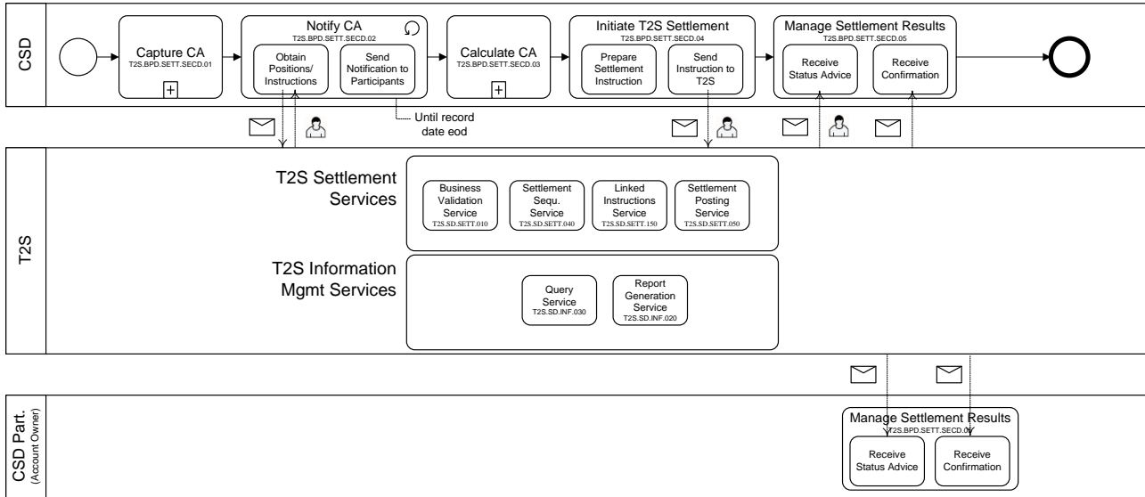
2 Figure 5-1: Business Process Diagram [T2S.BPD.SETT.SECD]
