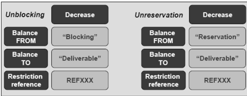
7 Figure 3-14: Enrich Settlement Restriction [T2S.BPD.SETT.UUCB.01.01]
