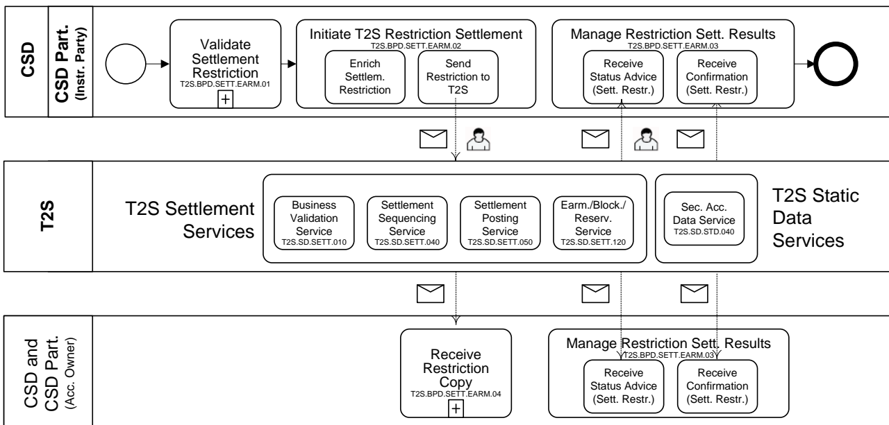
6 Figure 3-9: Business Process Diagram [T2S.BPD.SETT.EARM]
