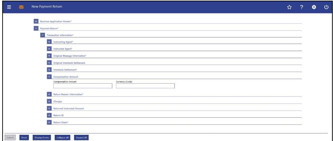
Figure 198 - Payment Return – New Screen – Compensation Amount
