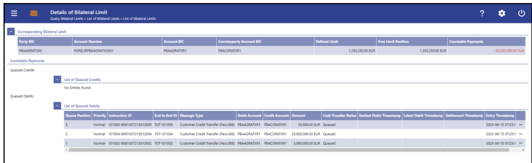
Figure 224 - Bilateral Limits – Details Screen
