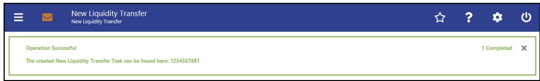
Figure 17 - Success Notification
