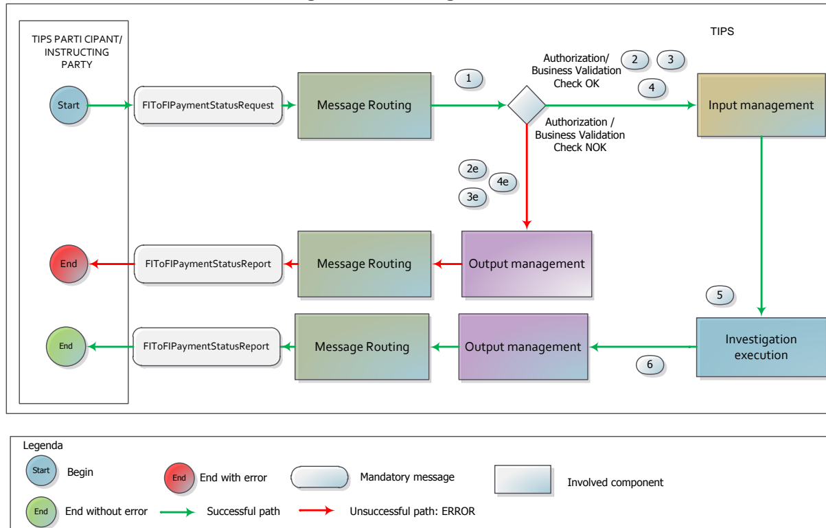
Figure 57 - Investigation Flow
