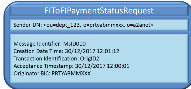
Figure 59 - Successful FIToFIPaymentStatusRequest
