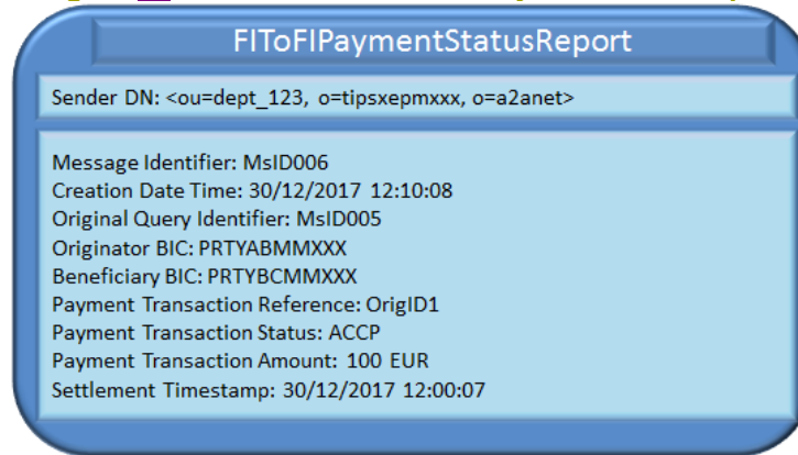
Figure 9061 - Successful FIToFIPaymentStatusReport
