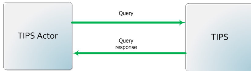
Figure 7775 -- Queries flow
