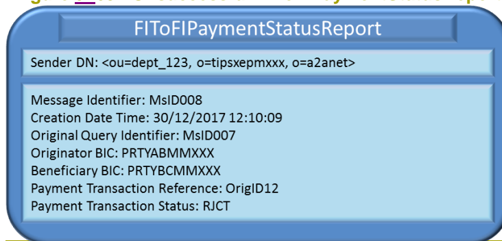
Figure 9263 - Unsuccessful FIToFIPaymentStatusReport
