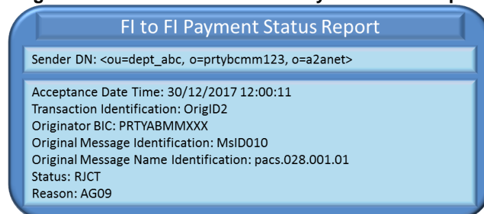
Figure 62 - Unsuccessful FIToFIPaymentStatusReport
