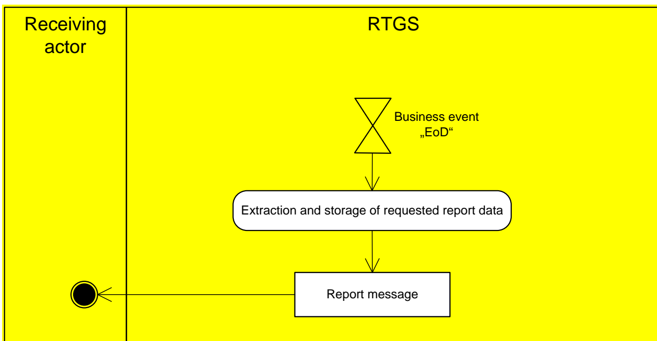
Figure 86 - RTGS receive report
