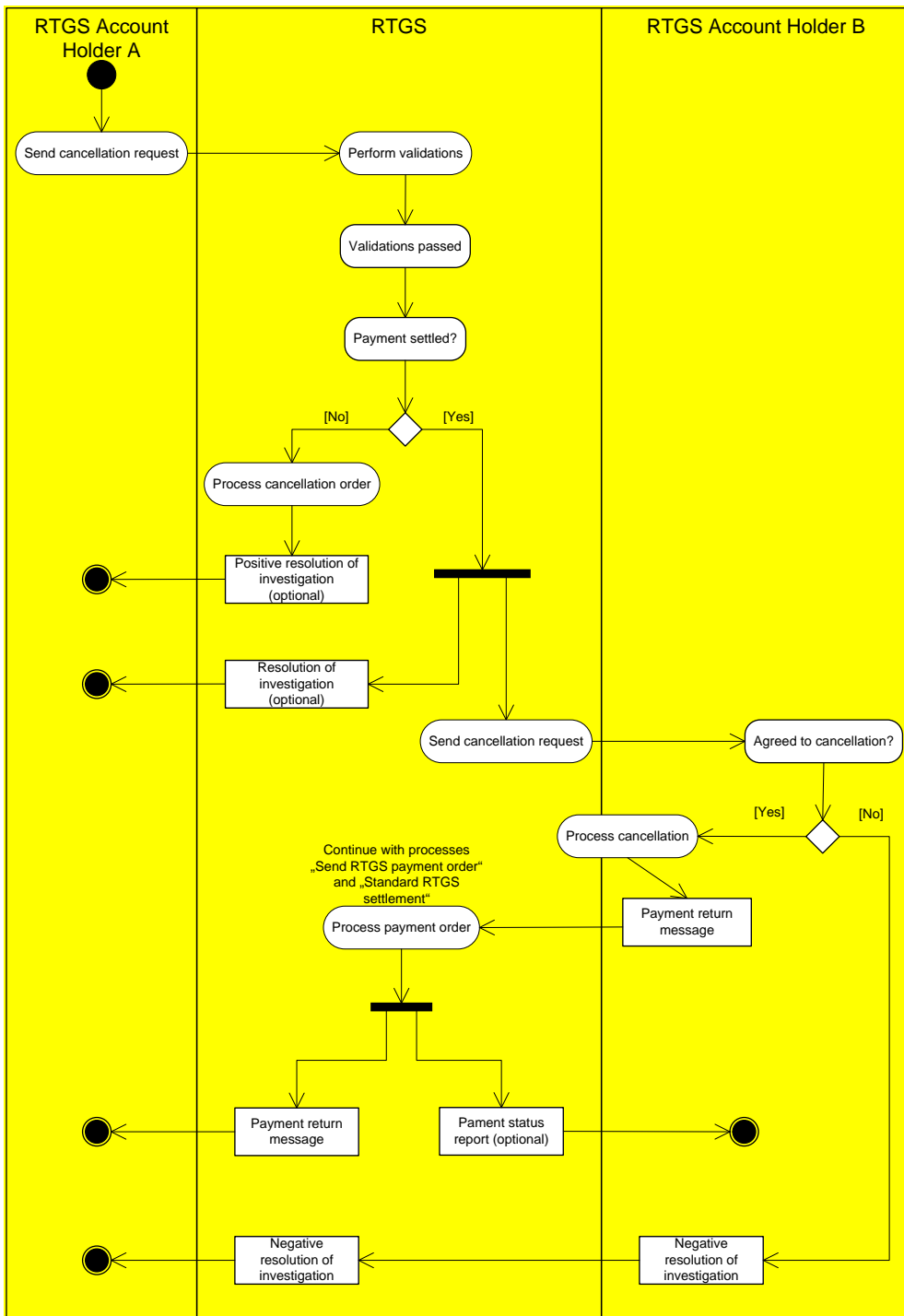
Figure 61 - Revoke/cancel payment
