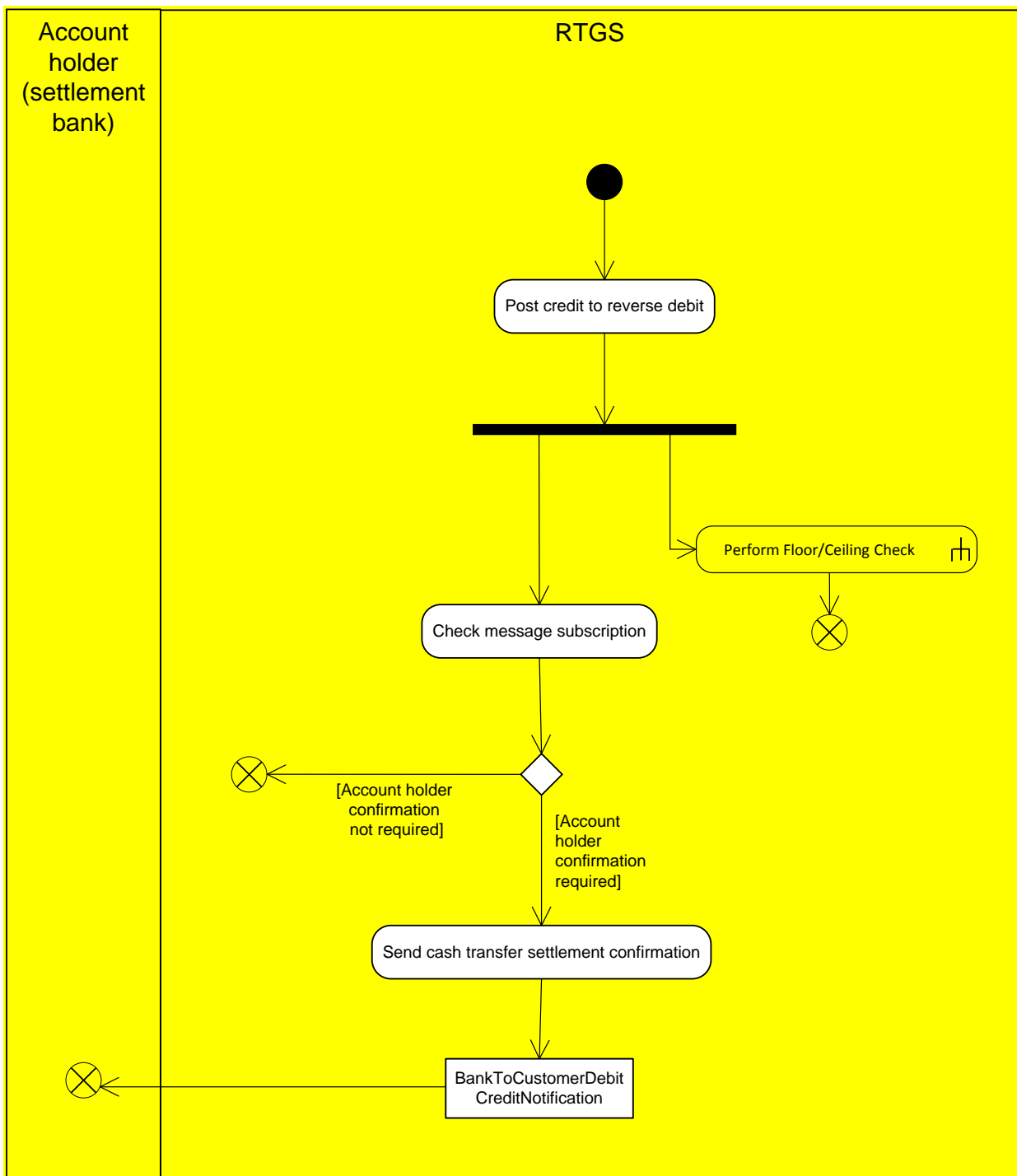
Figure 71 - Reverse debits
