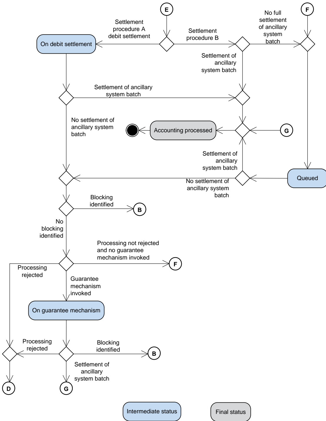
Figure 41 - Status transition diagram A and B
