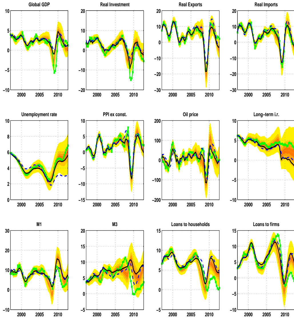
Figure 3: Conditional Forecasts
